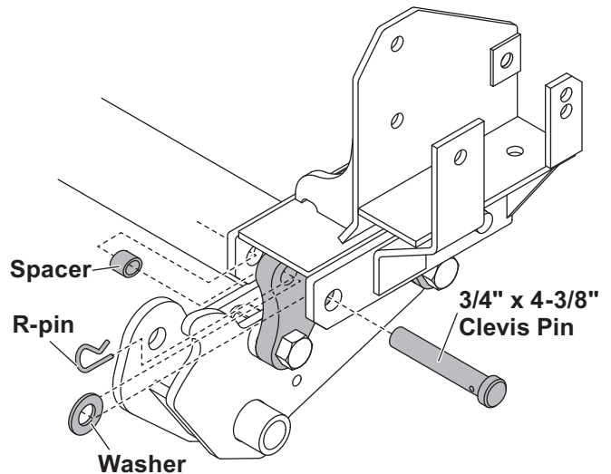
Shown with height adjustment plate installed
